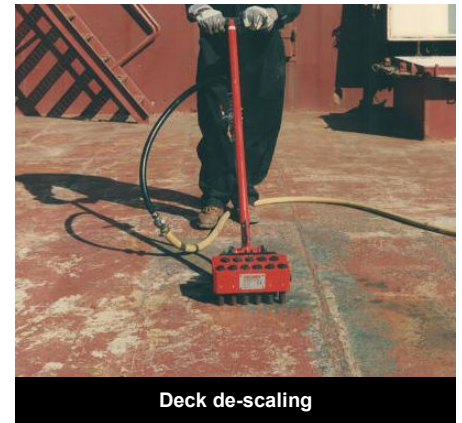
Deck de-scaling
